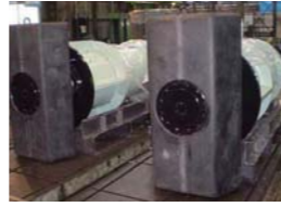
顶推驳船用连接装置 Taisei Engineering Consultants, Inc
